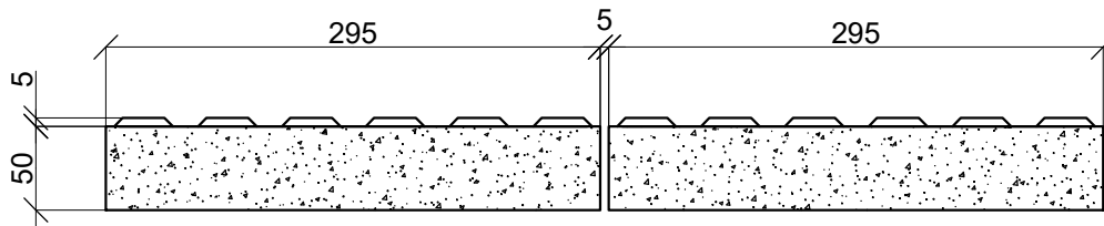
WARNING BLOCK 300 x 300 x 50mm THICK
