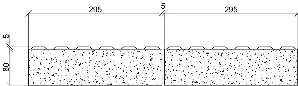
WARNING BLOCK 300 x 300 x 80mm THICK
