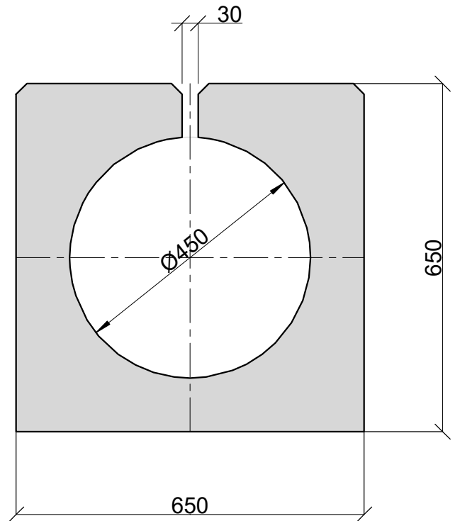
CROSS SECTION
