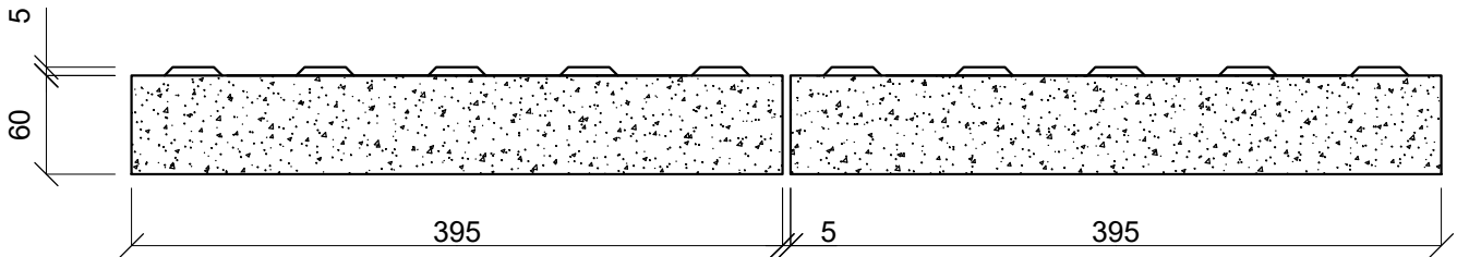
TACTILE DIRECTIONAL BLOCK 400 x 400 x 65mm THICK
