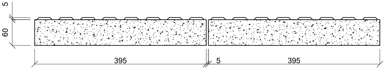
TACTILE WARNING BLOCK 400 x 400 x 65mm THICK
