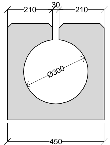
CROSS SECTION
